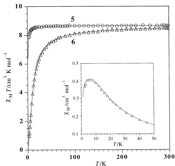
Fig. 7 Temperature dependence of \chi_{\text{m}}T of solid samples of complexes 5 and 6 (the solid line corresponds to the best fit). The inset shows the temperature variation of the susceptibility of 6 in the low-temperature region
