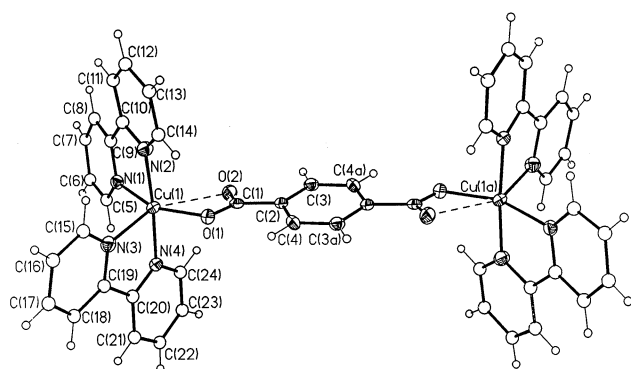
Fig. 1 Perspective view of the cationic unit [Cu 2 (bipy) 4 (ta)] 2+ of complex 1 showing the atom labelling. Thermal ellipsoids are drawn at the 30% probability level. The broken lines indicate the weak interaction between the Cu II and O(2) carbonyl oxygen of the co-ordinated carboxylate
