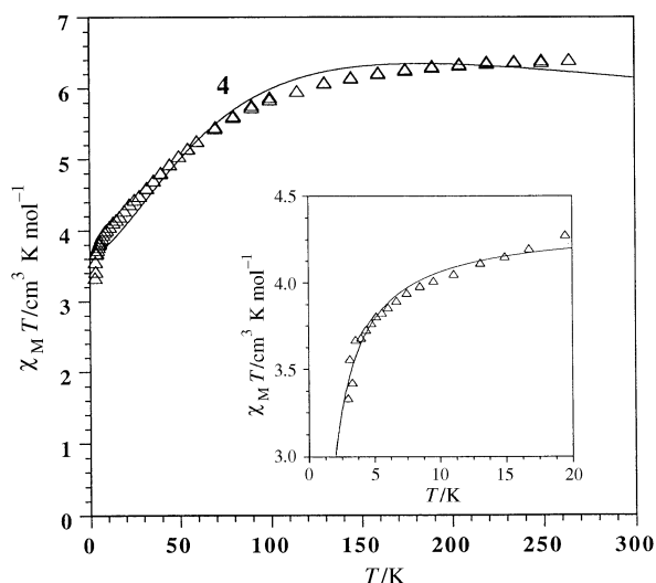
Fig. 6 Temperature dependence of \chi_{\text{m}}T of solid sample of complex 4. The solid line corresponds to the best fit through the Lines model (see text). The inset shows the low-temperature region and the solid line represents the best fit to the magnetic data for an Ising dimer ( S_{\text{eff}} = \frac{1}{2} )
