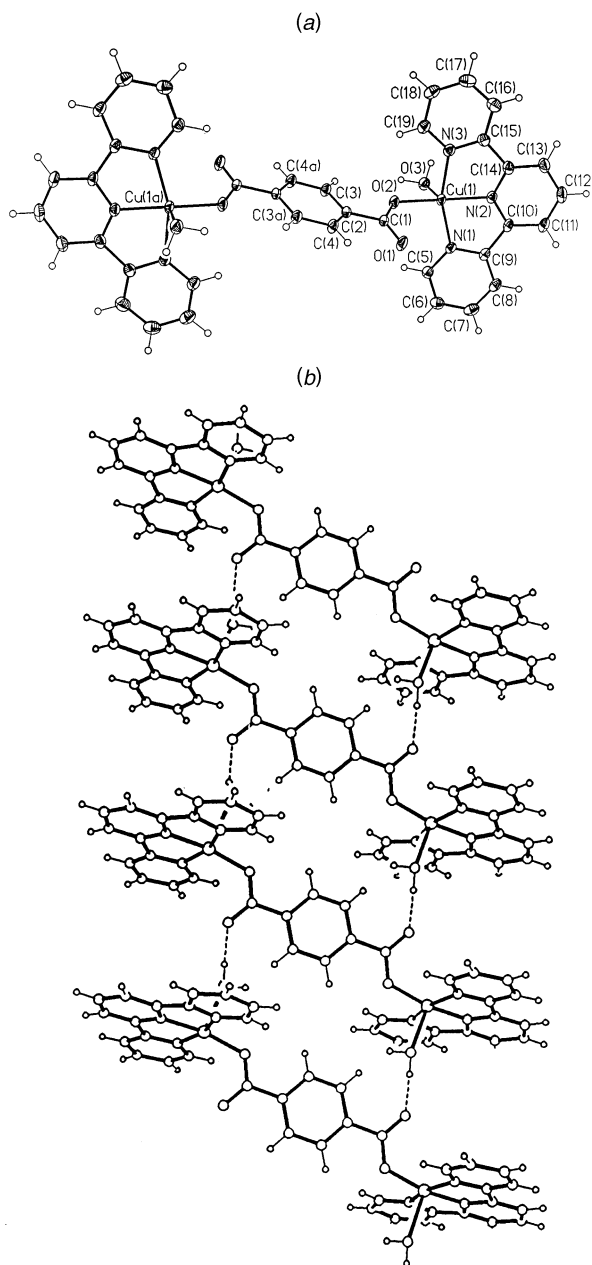
Fig. 2 (a) Perspective view of the cationic unit [\text{Cu}_2(\text{terpy})_2(\text{H}_2\text{O})_2(\text{ta})]^{2+} of complex 2 showing the atom labelling. Thermal ellipsoids are drawn at the 30% probability level. (b) A view of the intermolecular hydrogen bonding linking the dinuclear [\text{Cu}_2(\text{terpy})_2(\text{H}_2\text{O})_2(\text{ta})]^{2+} units
